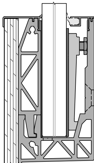
DECKUNG FRONT CF-112
