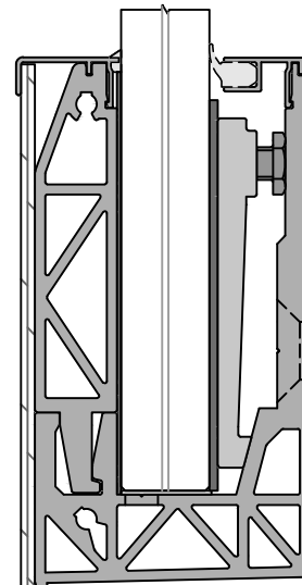
DECKUNG FRONT CF-103
