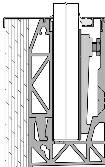
DECKUNG FRONT CF-120
