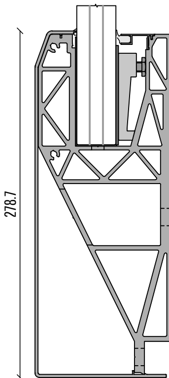
DECKUNG FRONT CF-312
