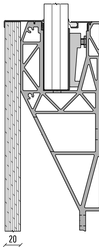
DECKUNG FRONT CF-320
