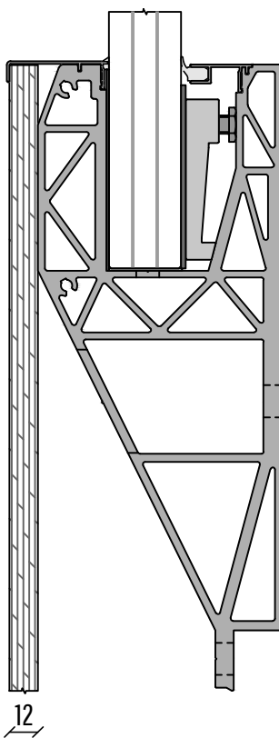
DECKUNG FRONT CF-312
